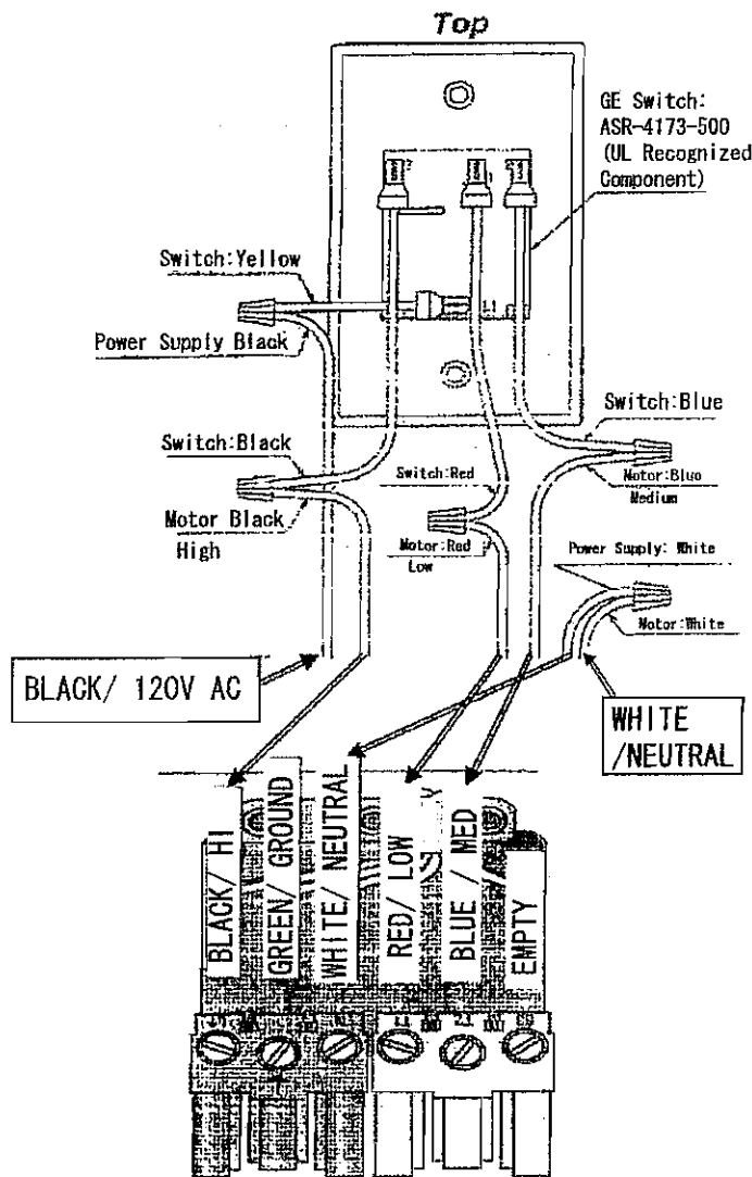
FIG 1 < Connection Diagram >
